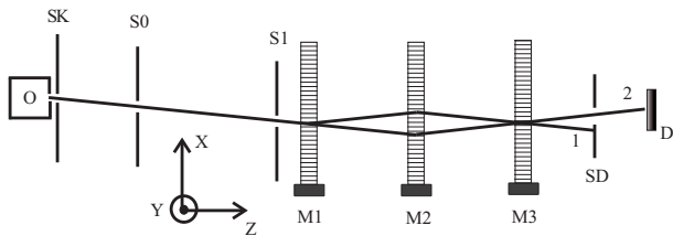
FIG. 1: Schematic drawing of a top view of our interferometer. The x, y, z axis are represented and, for each element, we give its distance z to the nozzle. O : lithium oven; Sk : 1 mm diameter skimmer at z_s = 15 mm ; S_0 : collimating slit of width w_0 = 20 \mu\text{m} at z_{S_0} = 480 mm; S_1 : collimating slit of width w_1 = 12 \mu\text{m} at z_{S_1} = 1260 mm; M_i, i = 1 - 3 : mirrors for the laser standing waves at z_{M_1} = 1410 mm, z_{M_2} = 2015 mm and z_{M_3} = 2620 mm; 1 and 2 : complementary exit beams; S_D : detector slit with tunable width and x-position at z_{S_D} = 3020 mm ; D : 760 \mu\text{m} wide rhenium ribbon of the Langmuir-Taylor hot wire detector at z_D = 3370 mm.
